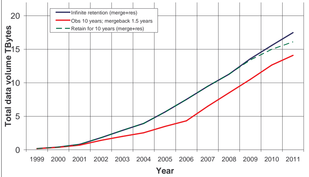
Figure 7. Accumulated satellite data volumes in MetDB archive for several options
