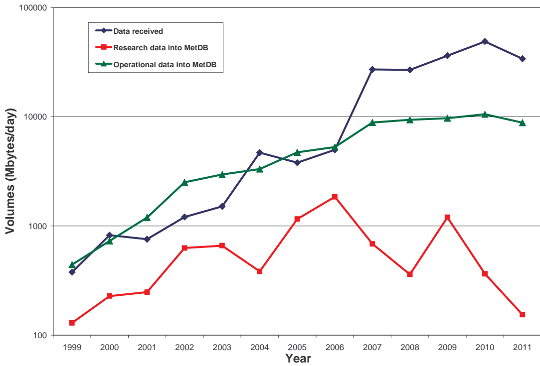
Figure 3. Daily data volumes entering Met Office
