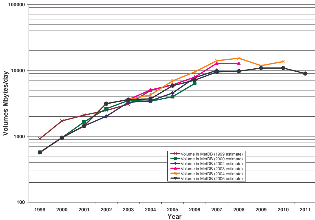
Figure 4: Projected satellite data volumes ingested into MetDB based on past and present best estimates (volumes based on input obs + mergeback + research files)
